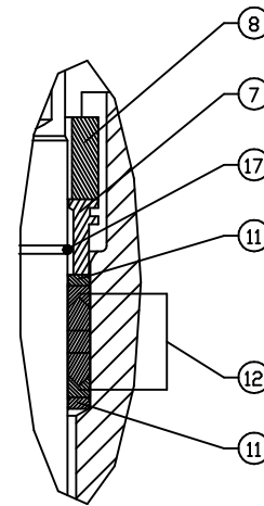
DETAIL A BRAIDED PACKING
