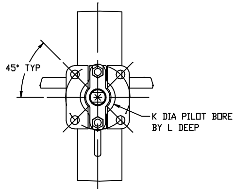
ISO MOUNTING
