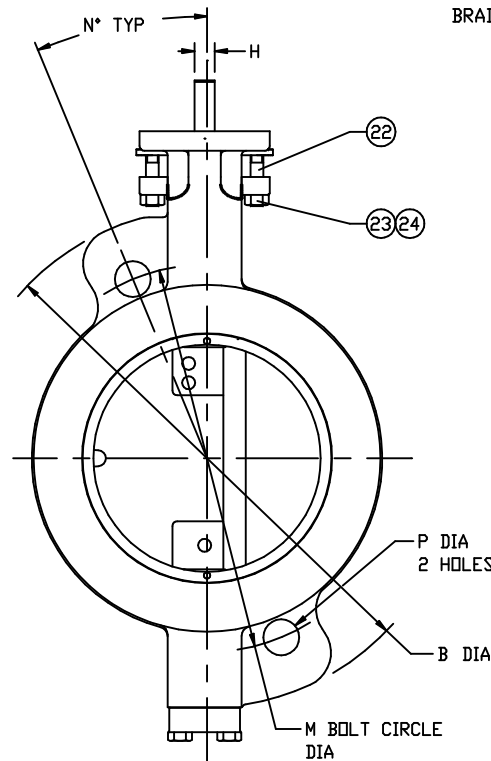
ISO MOUNTING
