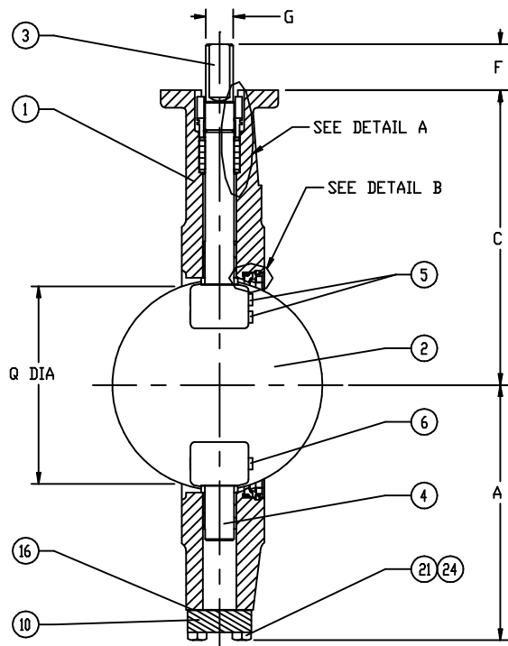
STANDARD MOUNTING
