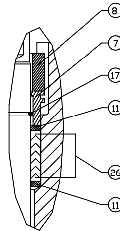
DETAIL A VEE-CUP
