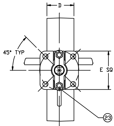
STANDARD MOUNTING
